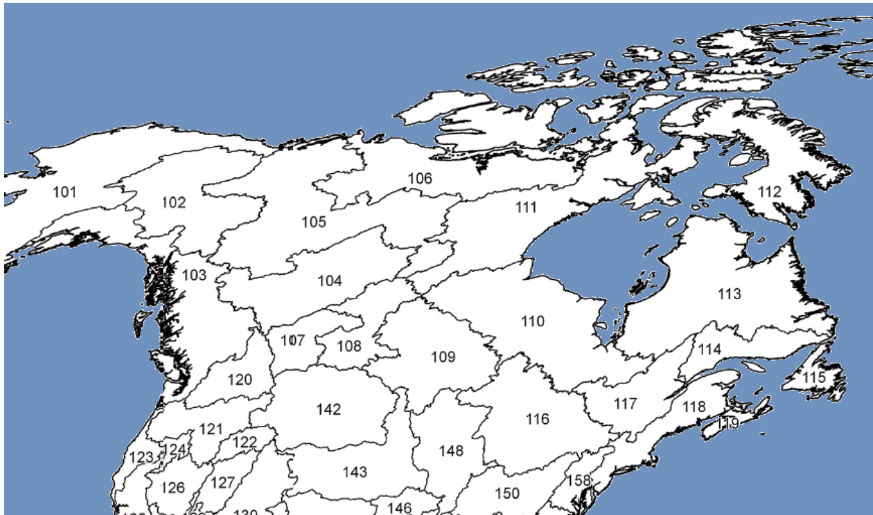
Figure 4. The freshwater ecoregions found in Canada. Note that the descriptions can be found in the source (Abell et al. 2008) and this figure has been modified from its original presentation.
