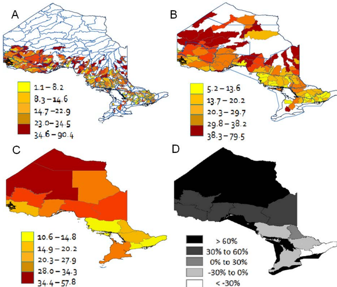
Figure 9. The lake Catch-Per-Unit-Effort of fish reported within quaternary (A) and tertiary (B) watersheds, and within FMZs (C). The percentage of overall fish production remaining in lakes within FMZs following the recreational fishery (D).
