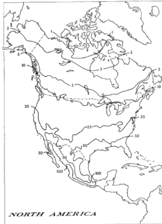
Figure 6. Isolines showing the upper limits to maximum sustainable fish yield (kg/ha/yr). Note coastal effects. Source: Schlesinger and Regier 1982.
