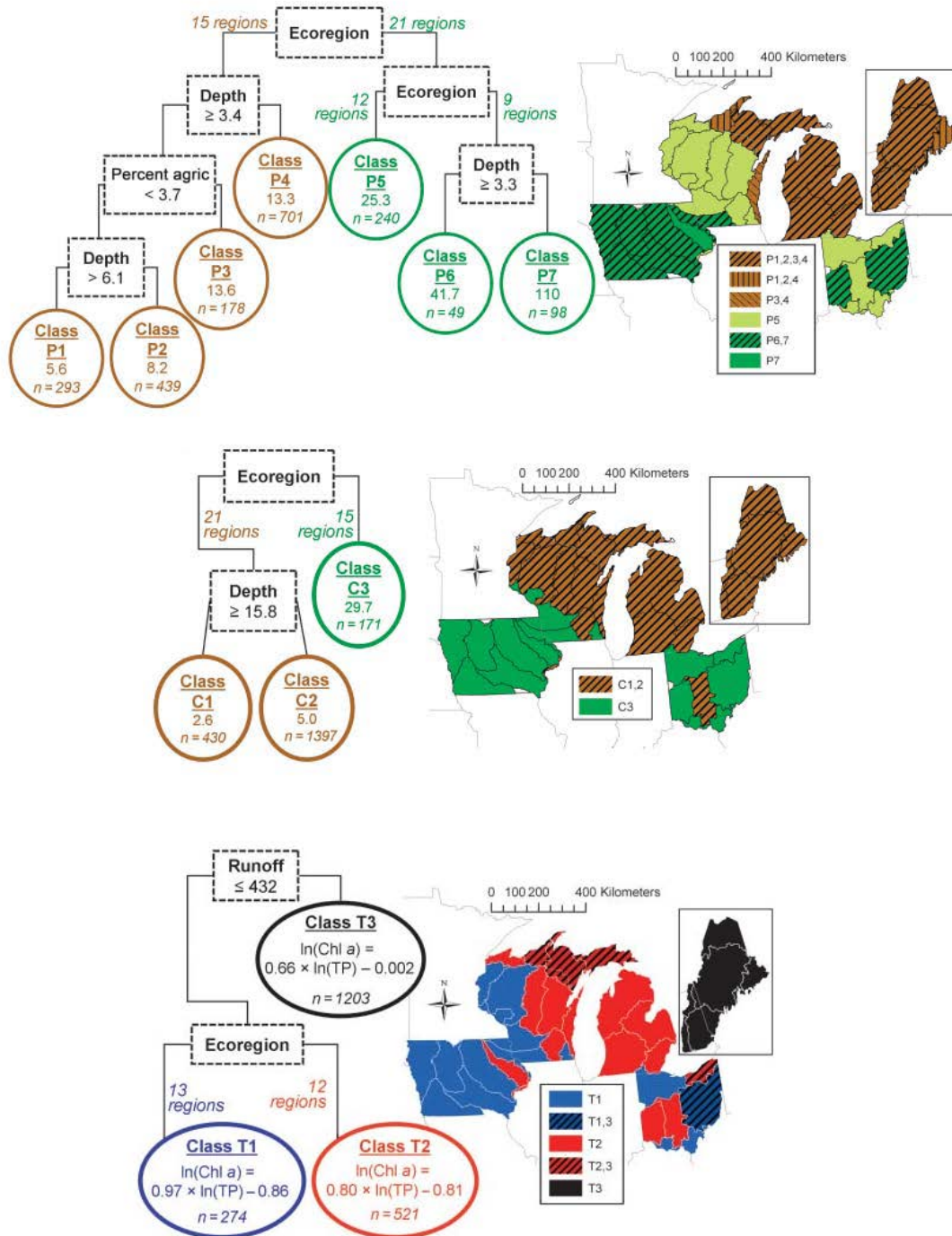
Figure 5. The classification trees (left) and maps (right) of areas within ecoregions that correspond to Total Phosphorus (top row) and Chlorophyll A (middle row) state variables, and a Total Phosphorus and Chlorophyll A response variable. (Source: Soranno et al. 2010, note that the Figure has been modified).
