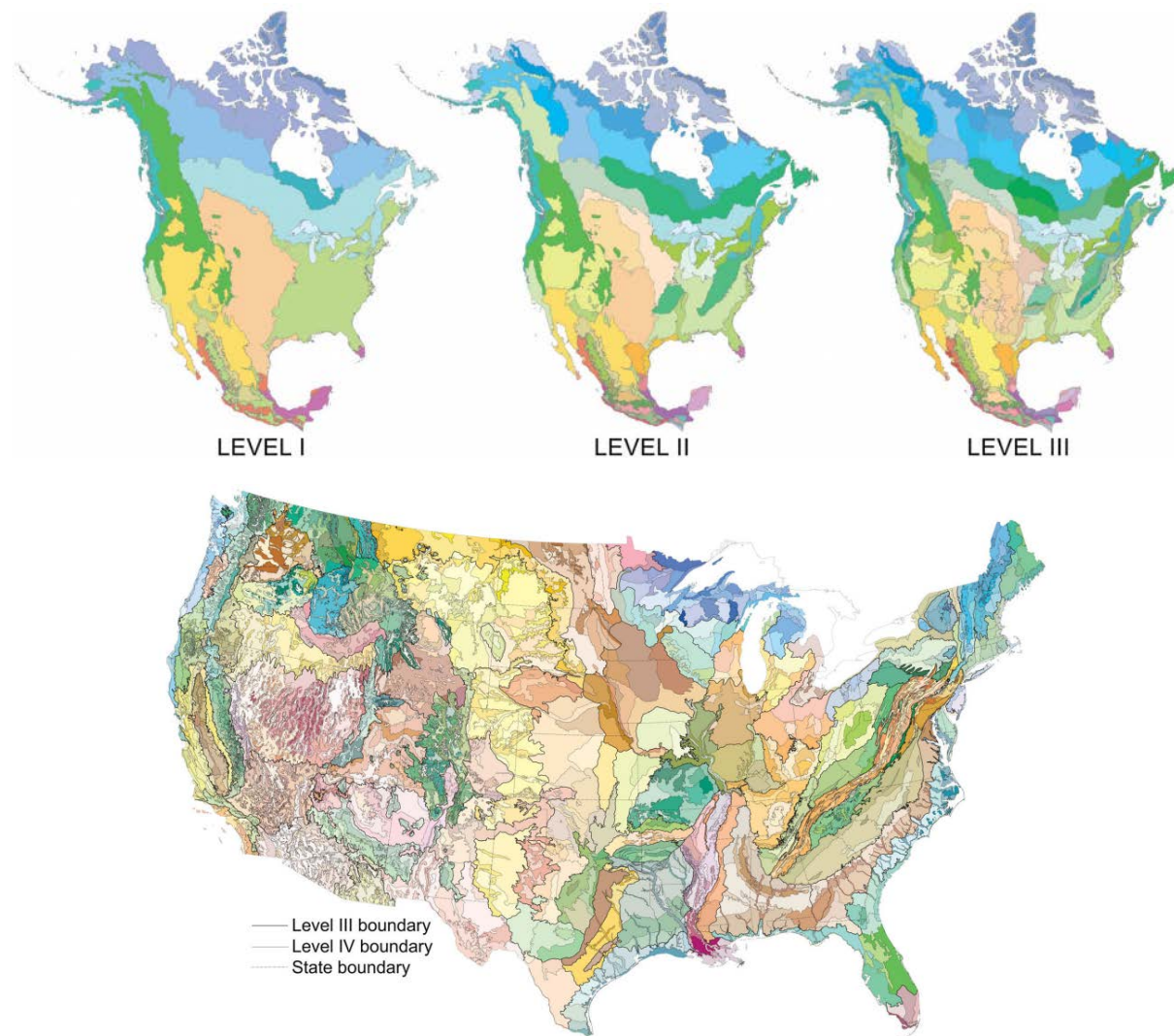
Figure 3. CEC and EPA Level I – III ecosystem classifications for North America (top row) and Level IV for the United States of America (Source: Omernik and Griffith 2014).
