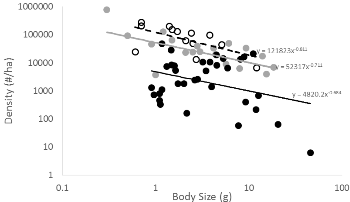
Figure 7. Relationships between the average body-size and the density of fish within a local community in Southern Canada and Europe (open circles), Northern Europe (grey circles) and the Lower Athabasca River tributaries (black circles).
